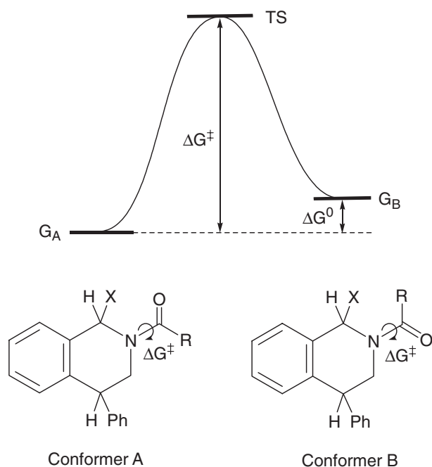
Figure 1. The rotational barrier and the conformational-energy difference between the conformers of N -substituted-4-phenyltetrahydroisoquinolines.
