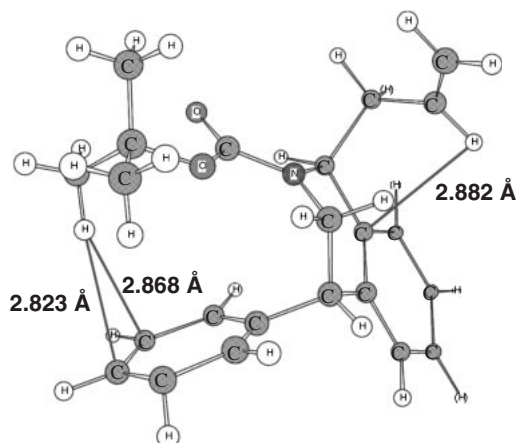
Figure 6. Optimized molecular structure of trans - 1 at MP2/6-31G(d,p) level.
