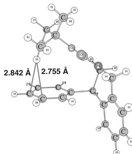
Figure 7. Optimized molecular structure of 4 at MP2/6-31G(d,p) level.
