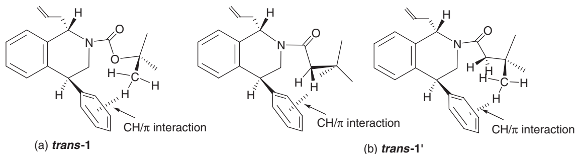
Figure 2. CH/ \pi interactions in (a) trans -1 and (b) trans -1'.
