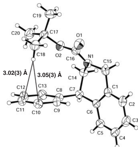
Figure 5. ORTEP drawing of 4 with thermal ellipsoids drawn at the 30% probability level. Selected C...H distances are shown in the Figure and values in parentheses are estimated standard deviations.
