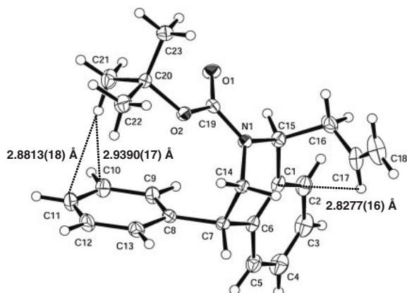
Figure 4. ORTEP drawing of trans - 1 with thermal ellipsoids drawn at the 30% probability level. Selected C...H distances are shown in the Figure and values in parentheses are estimated standard deviations.
