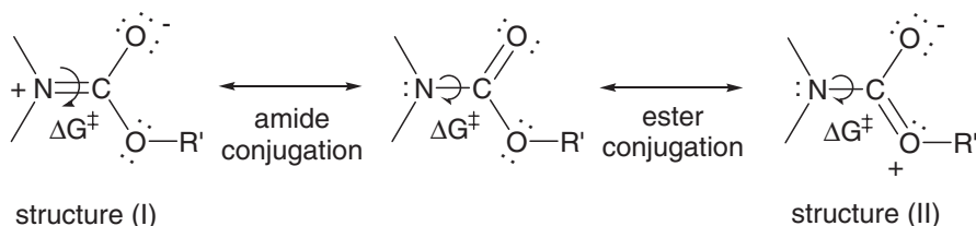
Figure 3. Cross conjugation in urethane.
